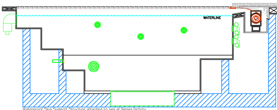
Waterproof Skid Support Structure attached to spa at Nespa factory
