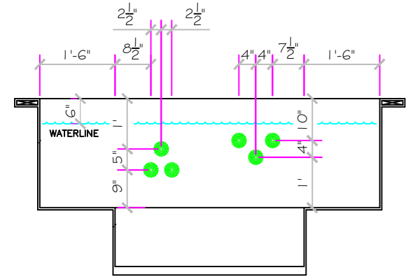
Section GK4
