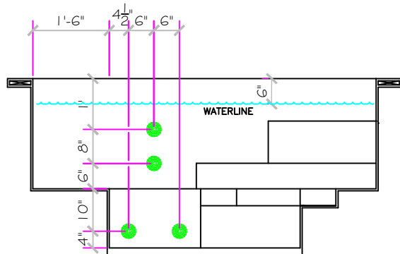
Section GK6
