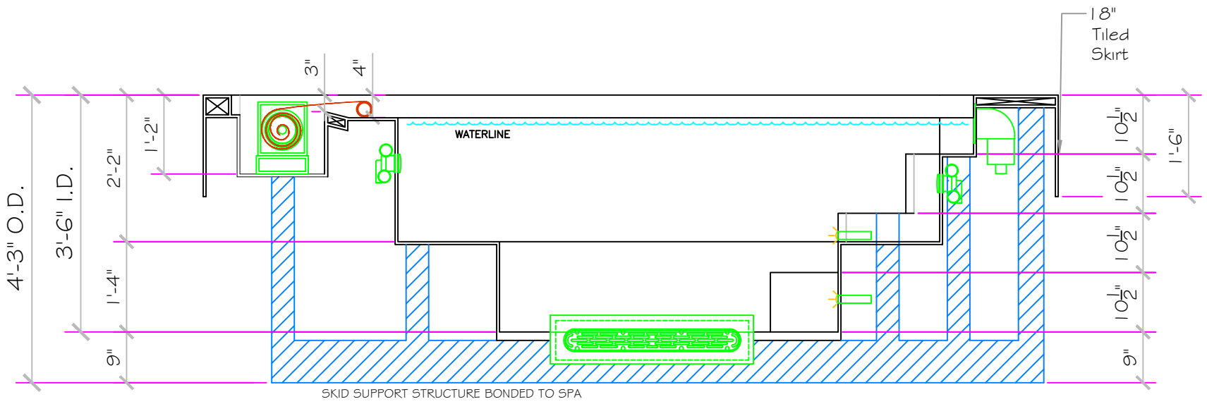
SECTION B-B
